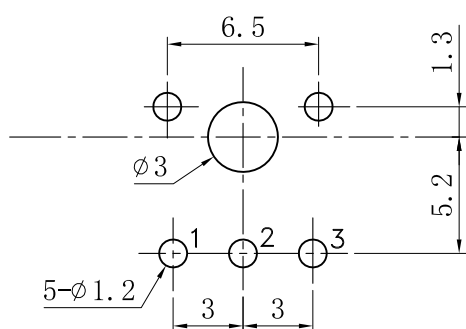
Mounting Hole
