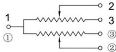
Circuit explanation:N0
