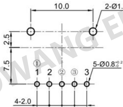
P.C.B. mounting hole detail
