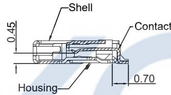
Section:A-A Scale:2/1
