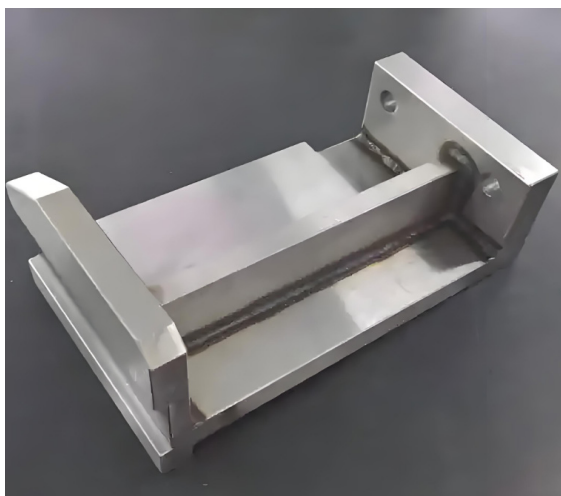
Welded assembly
